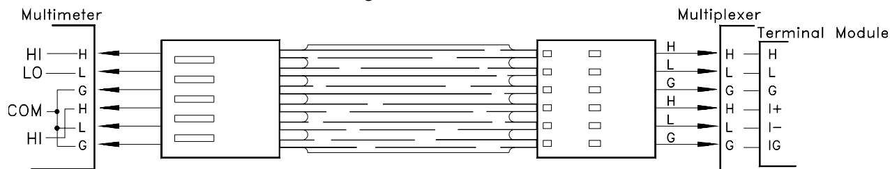
Figure 2-9. Analog Bus Connections
