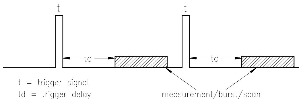
Figure 4-2. Multimeter Trigger Delays
